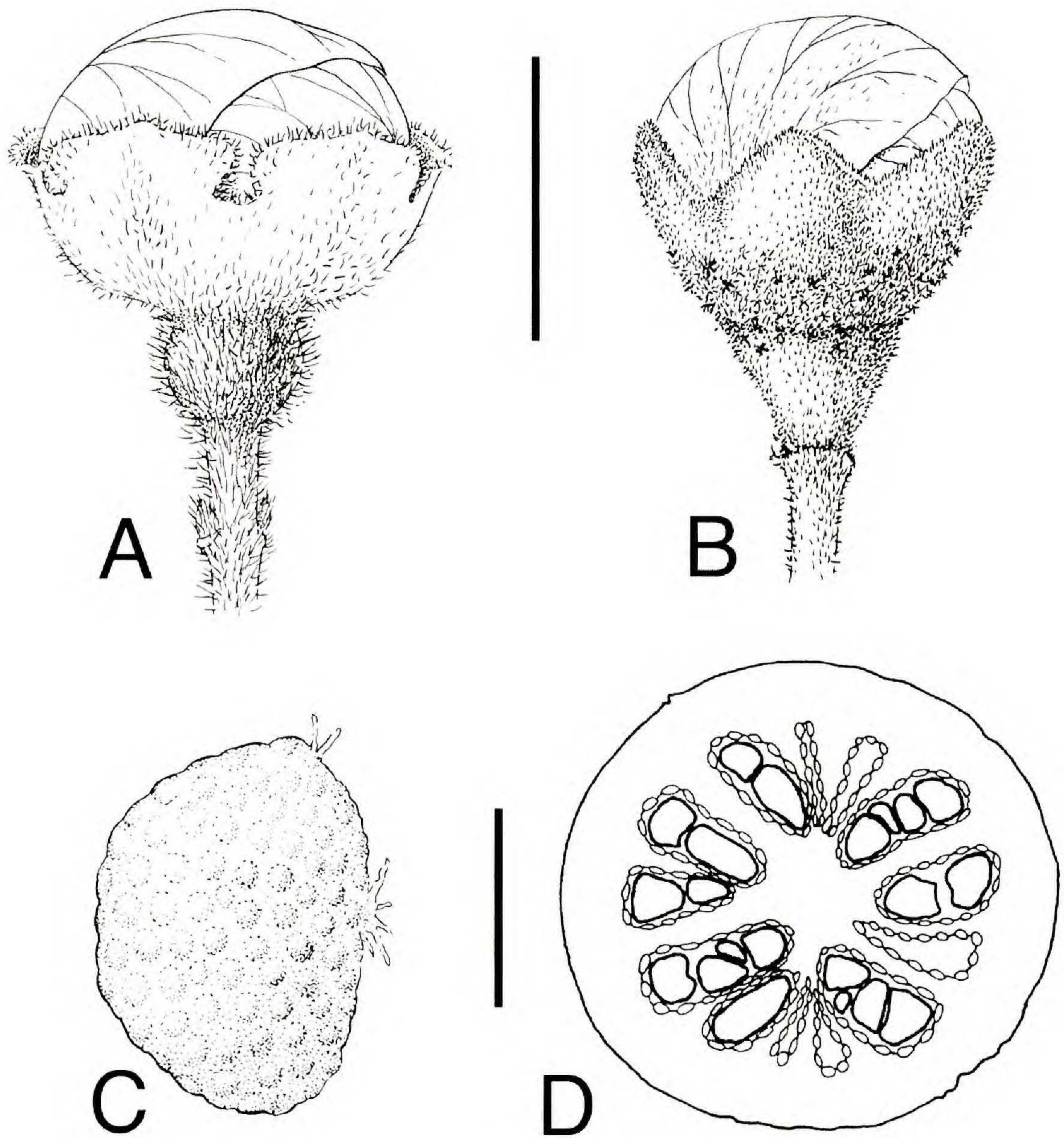
FIG. 1. A, Flower bud of Campomanesia viatoris . B, Flower bud of C. guaviroba . C, Locule containing a seed showing the glandular locular wall that serves as a false seed coat. D, Cross section of a fruit having 13 locules, each with a glandular wall, but only 8 of which contain seeds. Because the embryos are spiral in form, in section they may be cut in more than one place. Upper bar = 5 mm for A & B. Lower bar = 4 mm for C and 10 mm for D.
